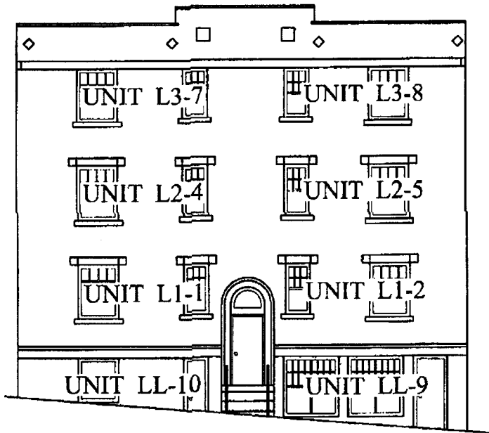
EAST ELEVATION
